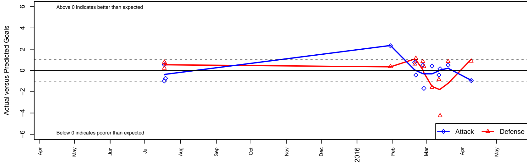
Tracyton Synergy G99 Dots are actual minus expected GF (blue circles) and GA (red triangles). Blue line is smoothed change in attack strength. Red is smoothed change in defense strength.
